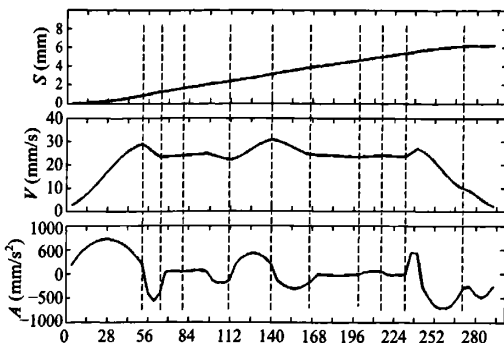
Fig.5 Results of displacement, speed and acceleration curve
