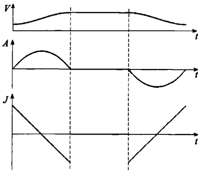
Fig.1 Speed ( V ), acceleration ( A ) and jerk ( J ) of the cubic polynomial acc/dec control model
