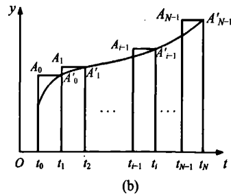
Fig.2 Implement curve of f(t) . (a) Left endpoints used for the heights of rectangles; (b) Right endpoints used for the heights of rectangles
