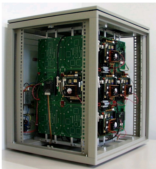
Figure 7: parallel main computer used to control the KDH II
